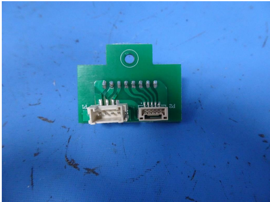
Charging PCB
