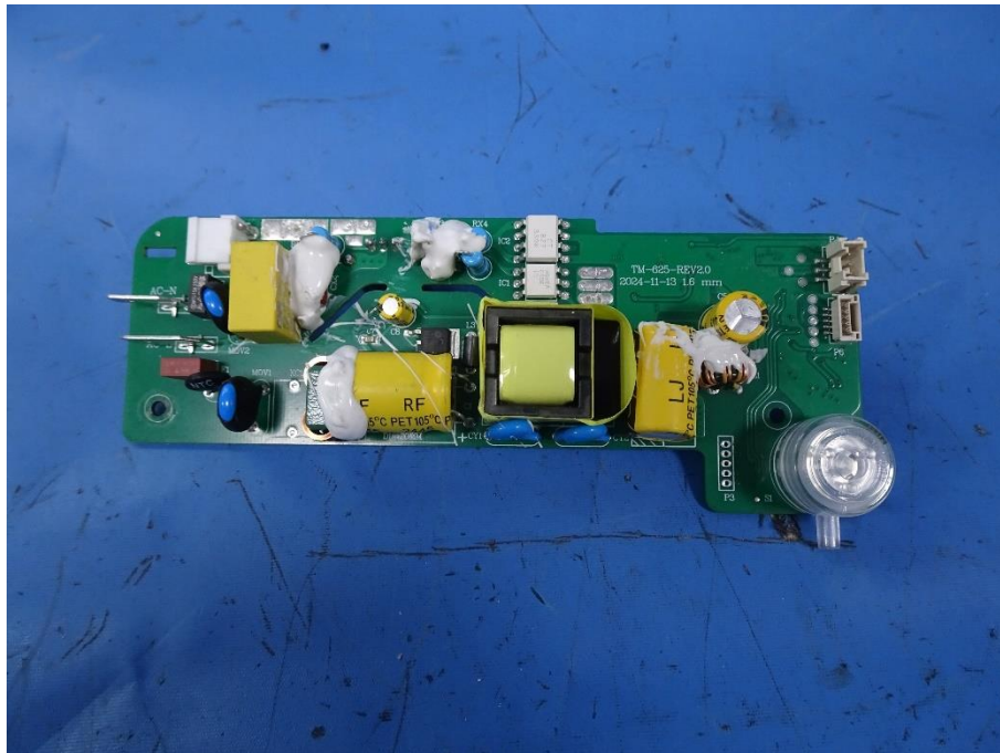
Main PCB
